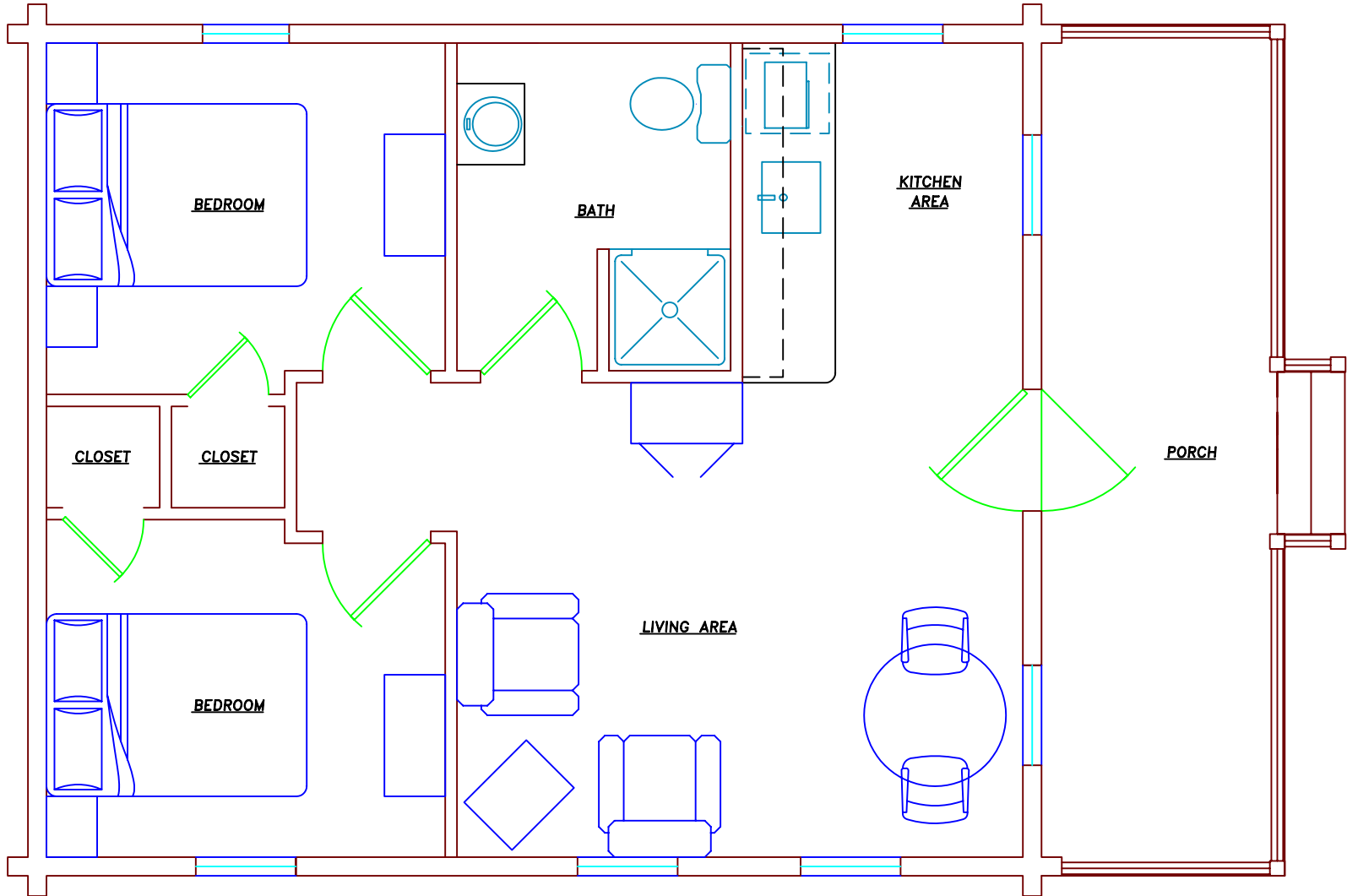
CABIN "B" FLOOR PLAN 10
